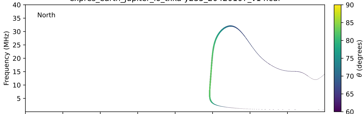
expres_earth_jupiter_io_txka-y235_20420107_v14.cdf
