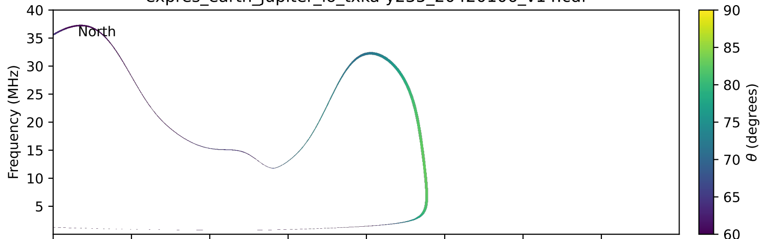
expres_earth_jupiter_io_txka-y235_20420106_v14.cdf
