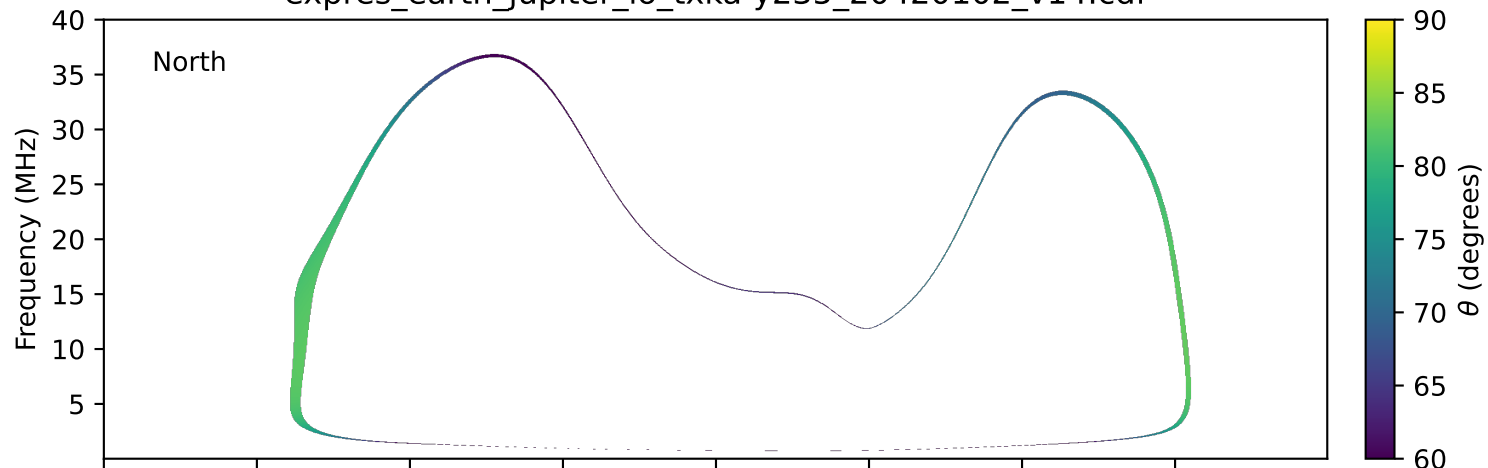
expres_earth_jupiter_io_txka-y235_20420102_v14.cdf
