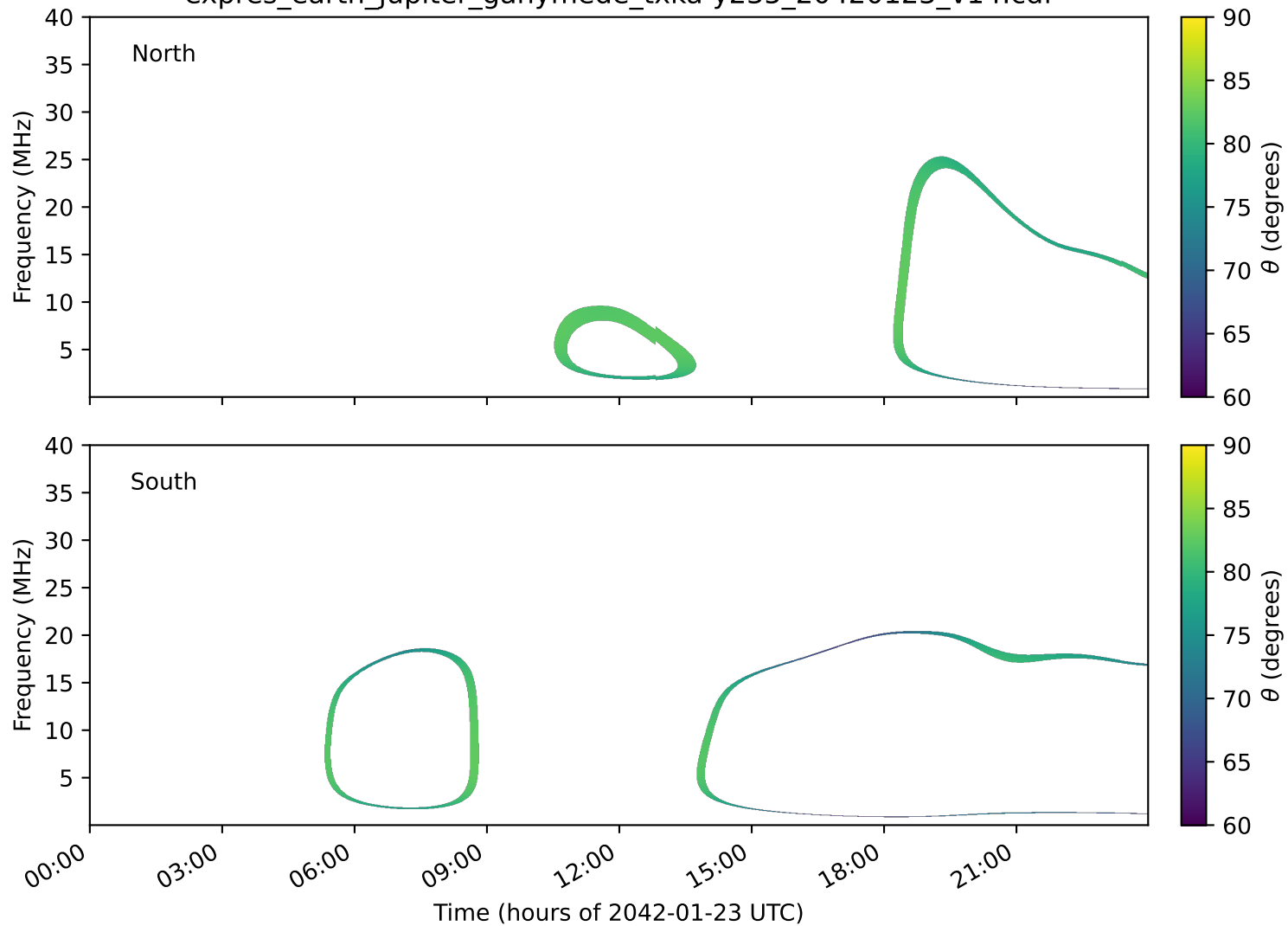
expres_earth_jupiter_ganymede_txka-y235_20420123_v14.cdf
