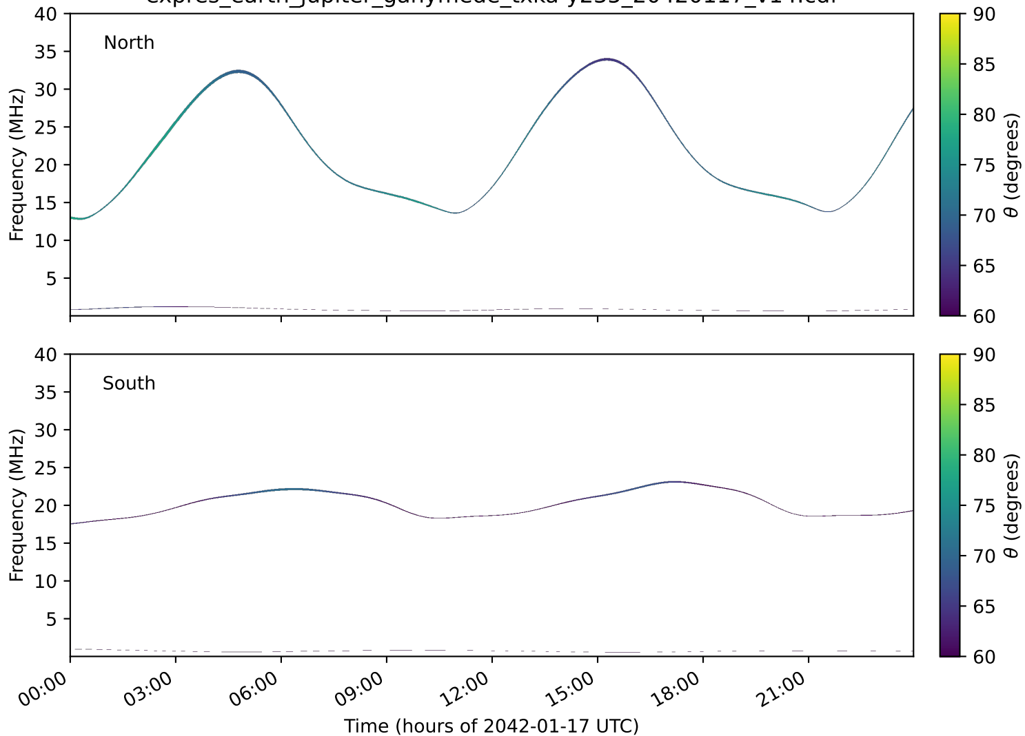
expres_earth_jupiter_ganymede_txka-y235_20420117_v14.cdf
