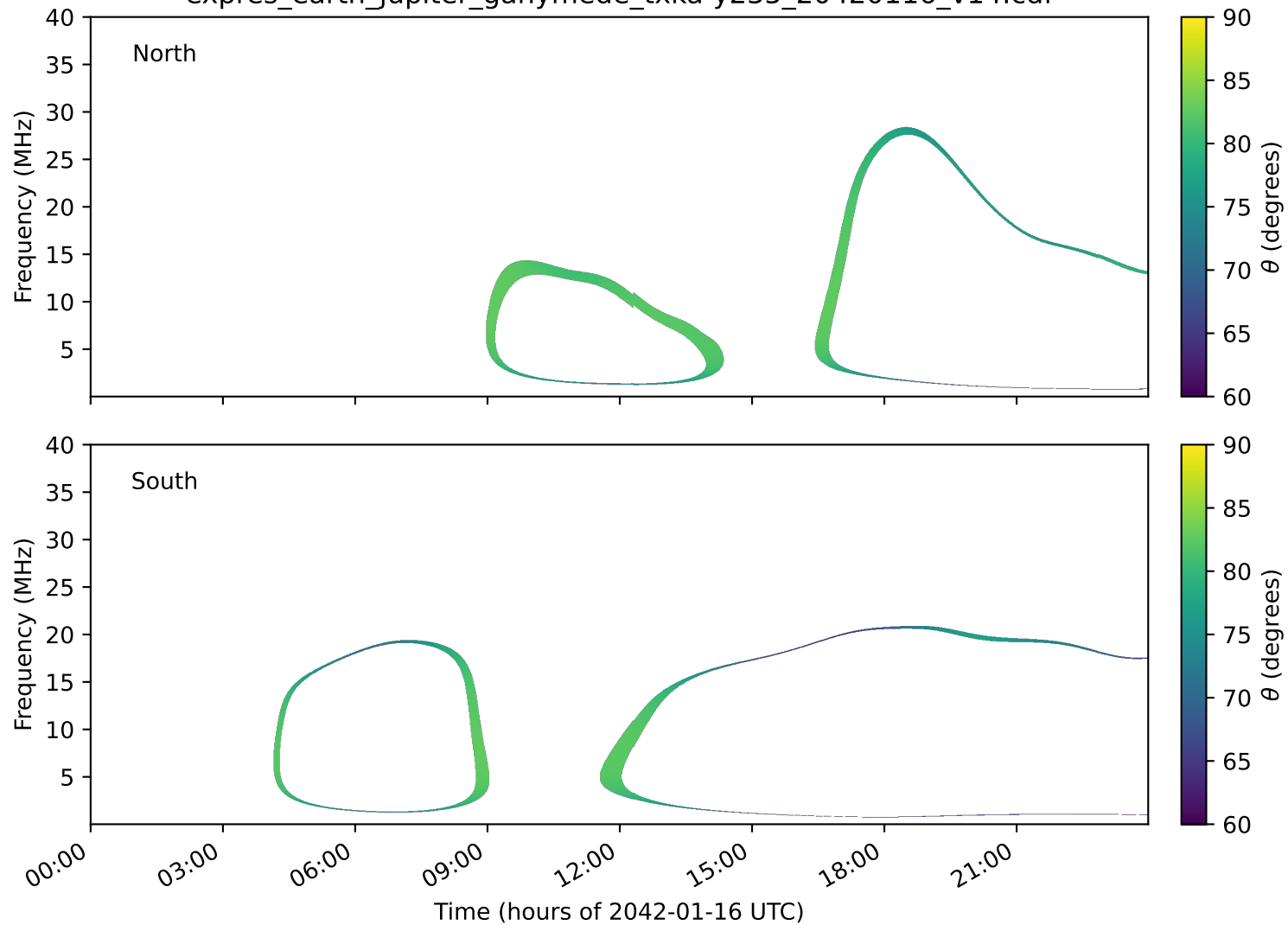
expres_earth_jupiter_ganymede_txka-y235_20420116_v14.cdf
