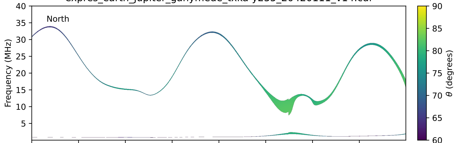
expres_earth_jupiter_ganymede_txka-y235_20420111_v14.cdf
