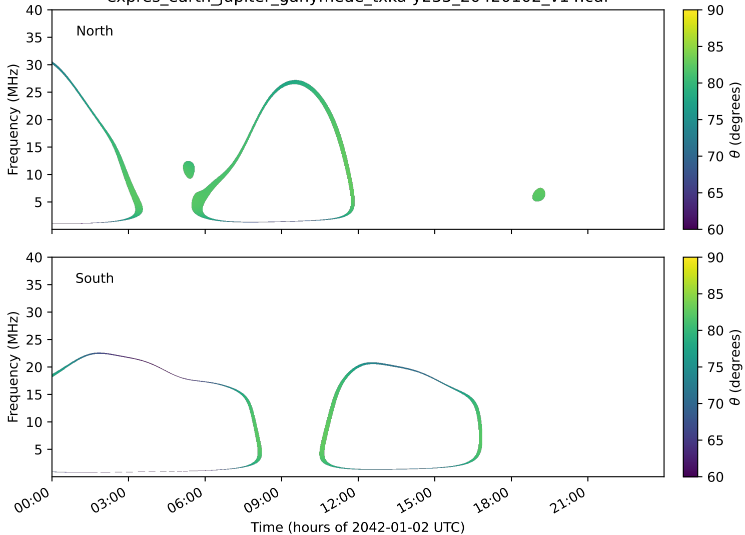
expres_earth_jupiter_ganymede_txka-y235_20420102_v14.cdf
