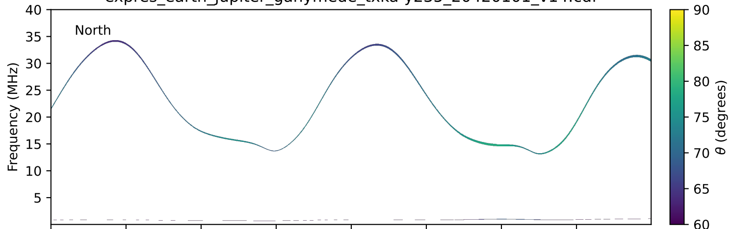
expres_earth_jupiter_ganymede_txka-y235_20420101_v14.cdf
