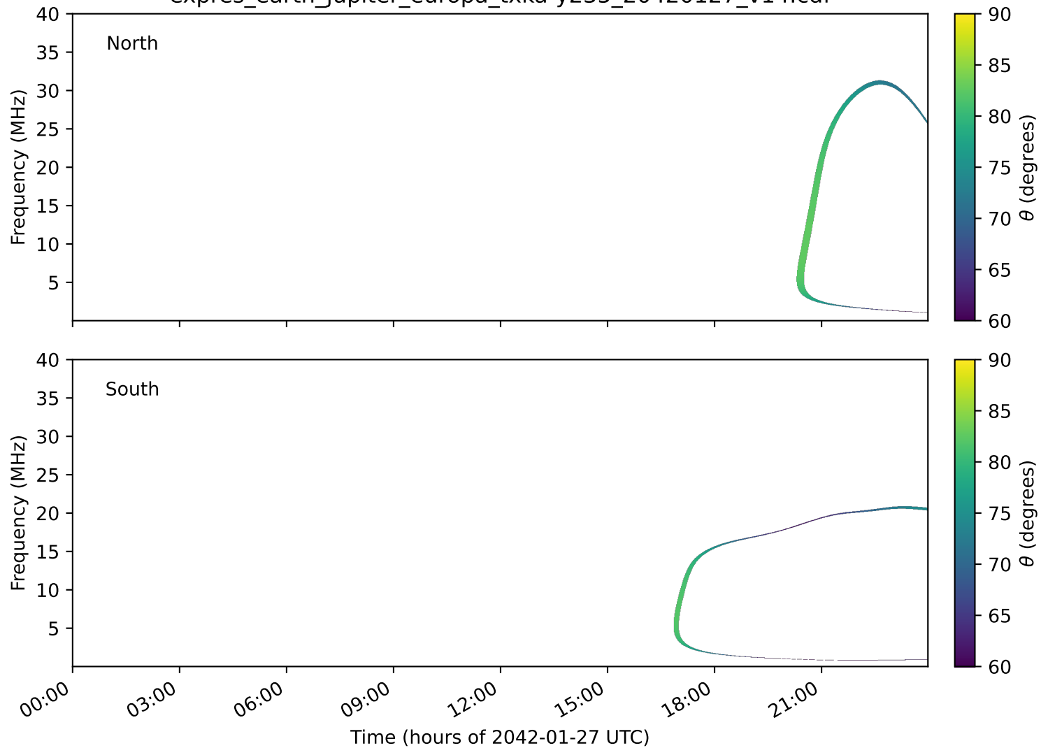
expres_earth_jupiter_europa_txka-y235_20420127_v14.cdf
