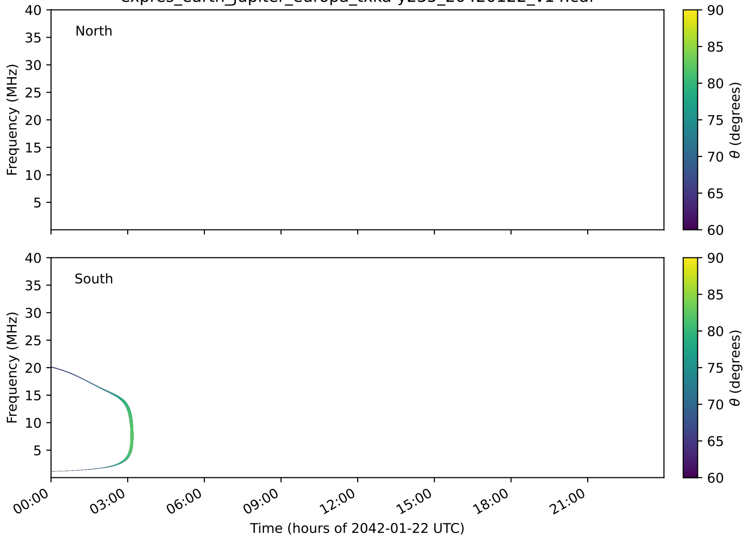
expres_earth_jupiter_europa_txka-y235_20420122_v14.cdf
