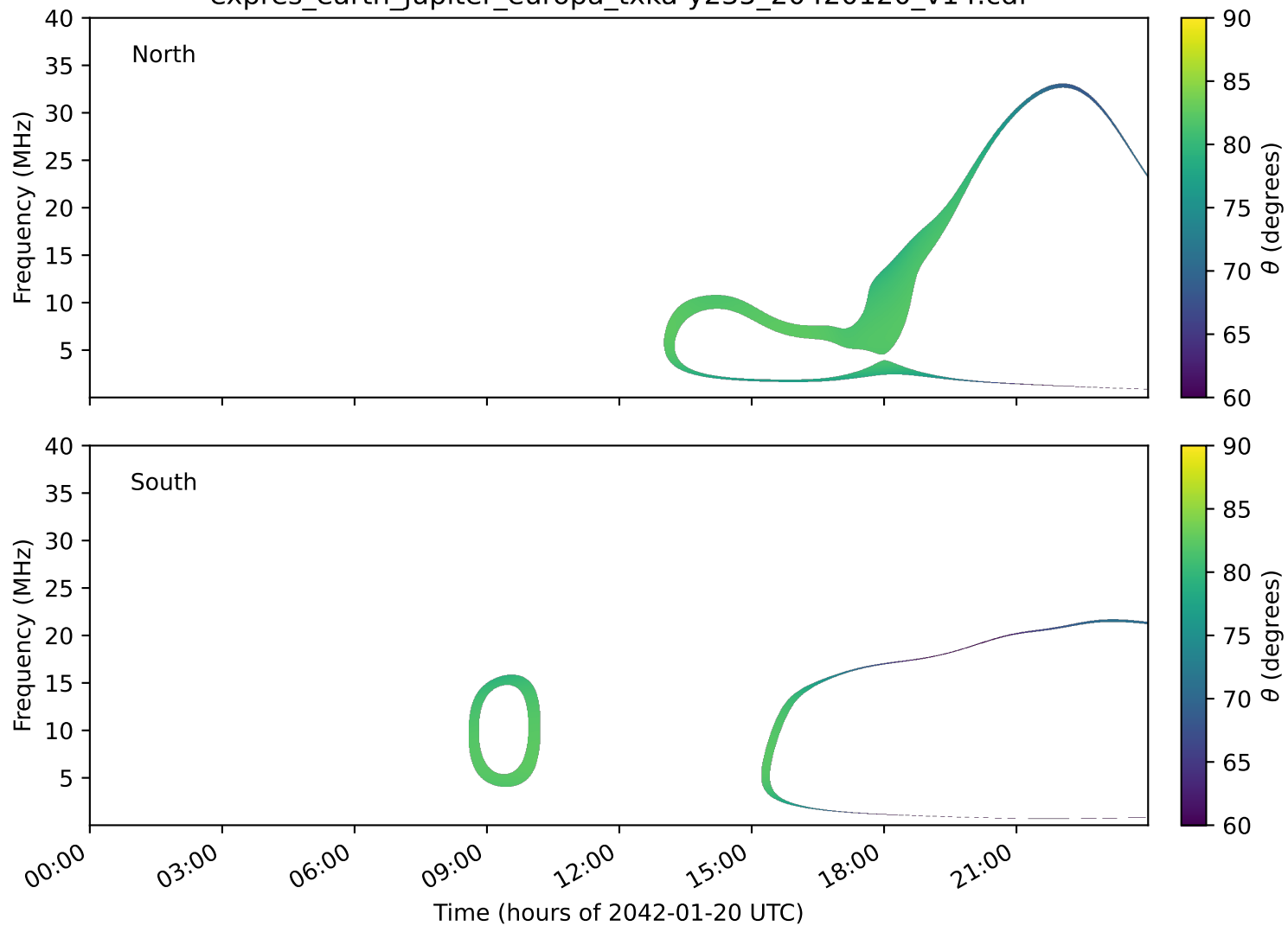
expres_earth_jupiter_europa_txka-y235_20420120_v14.cdf
