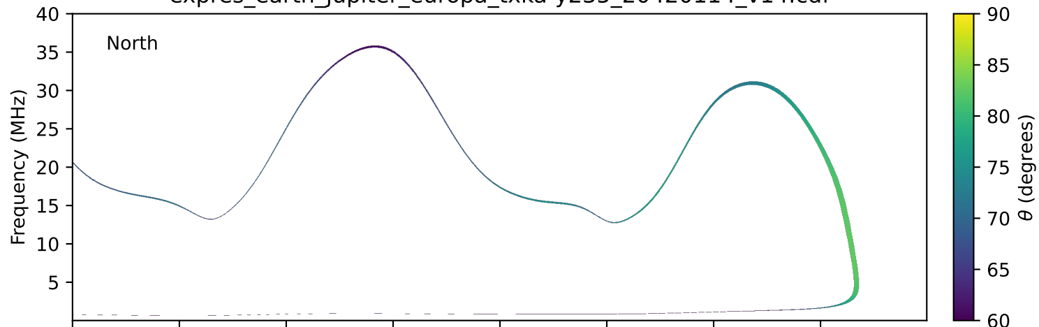
expres_earth_jupiter_europa_txka-y235_20420114_v14.cdf
