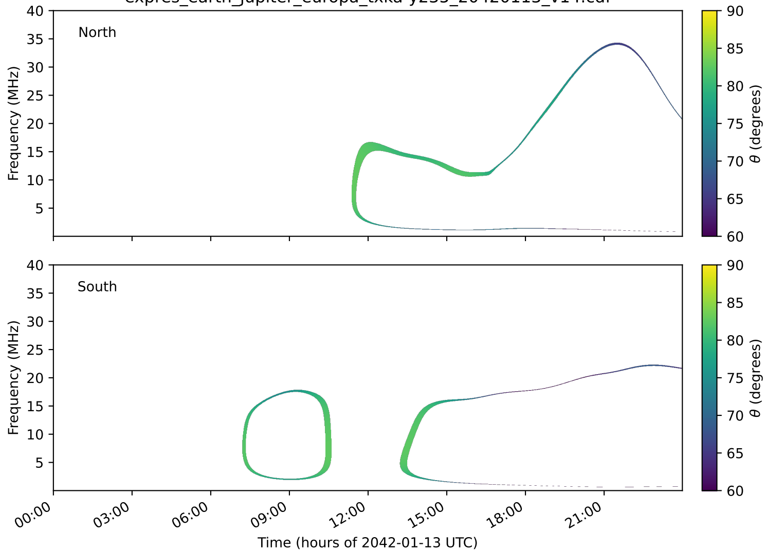
expres_earth_jupiter_europa_txka-y235_20420113_v14.cdf
