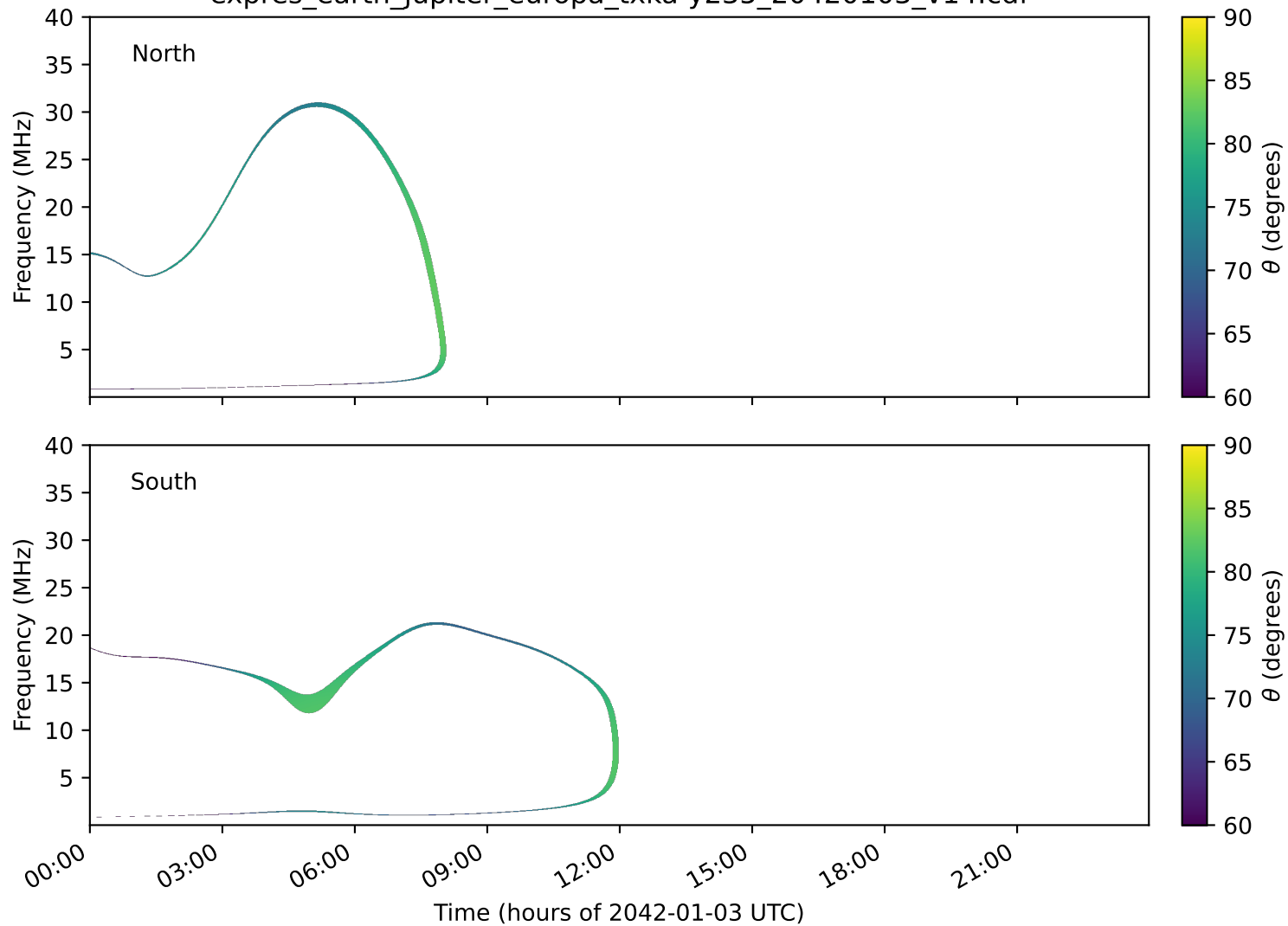
expres_earth_jupiter_europa_txka-y235_20420103_v14.cdf
