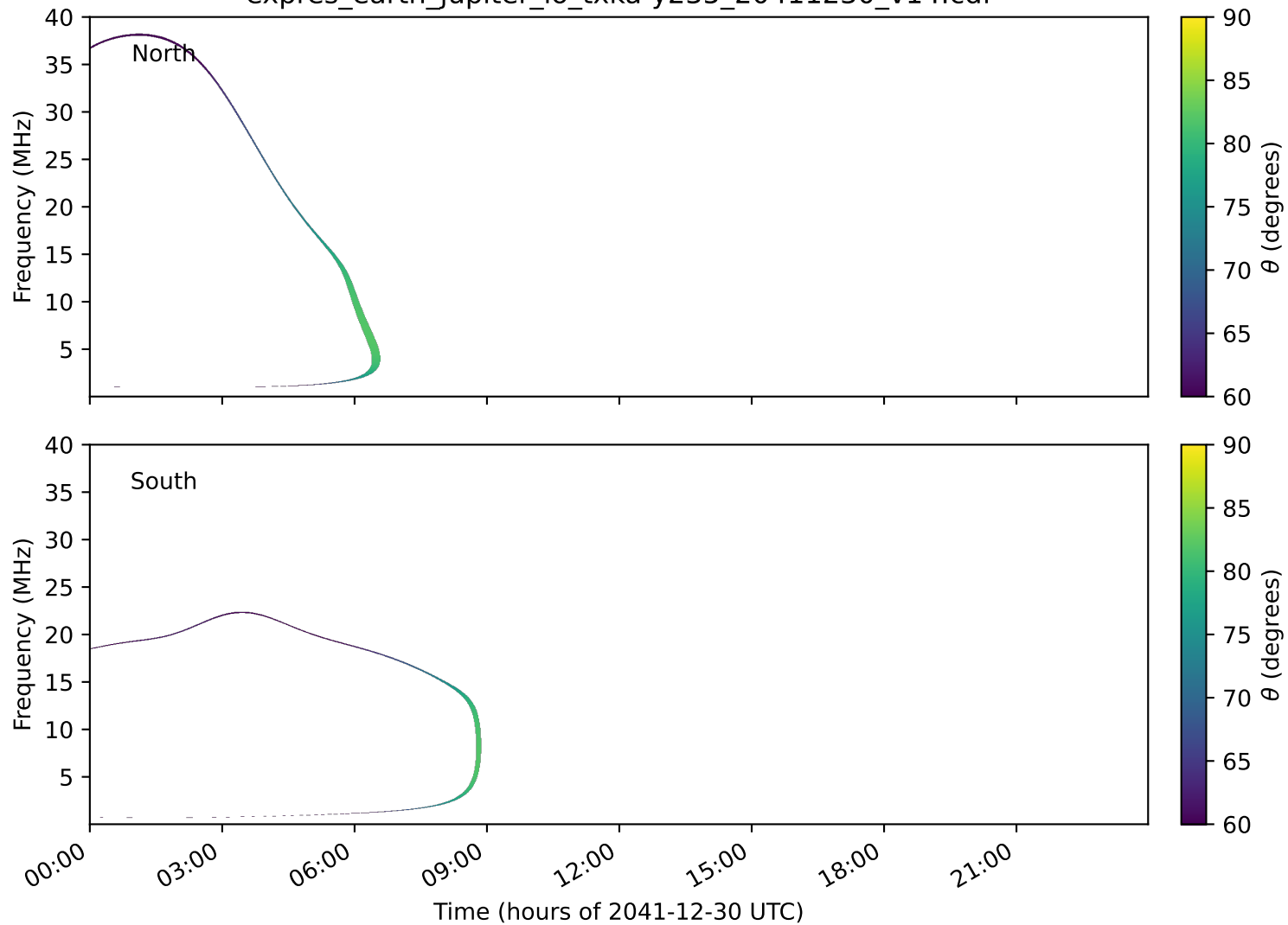
expres_earth_jupiter_io_txka-y235_20411230_v14.cdf
