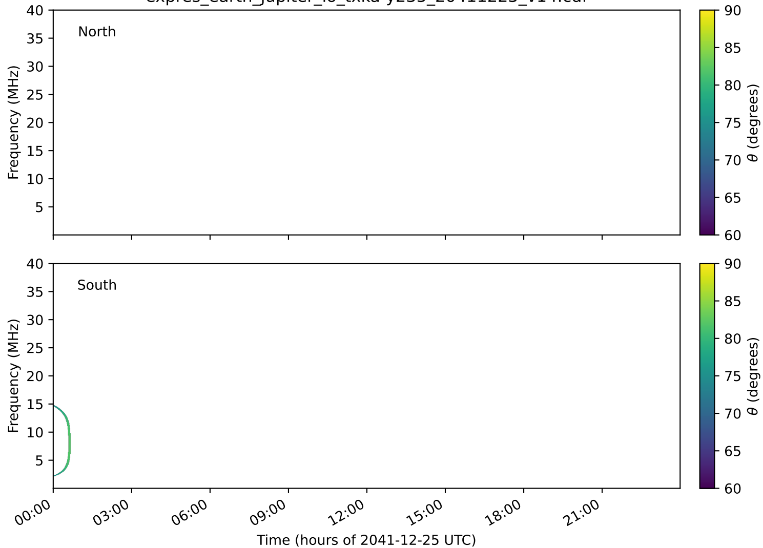
expres_earth_jupiter_io_txka-y235_20411225_v14.cdf
