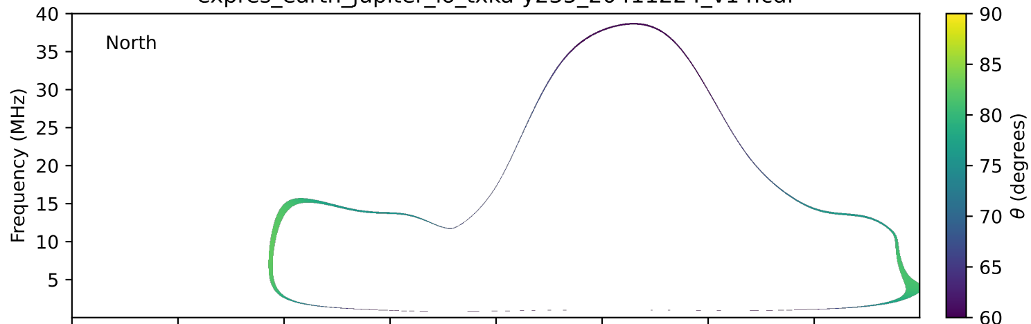
expres_earth_jupiter_io_txka-y235_20411224_v14.cdf
