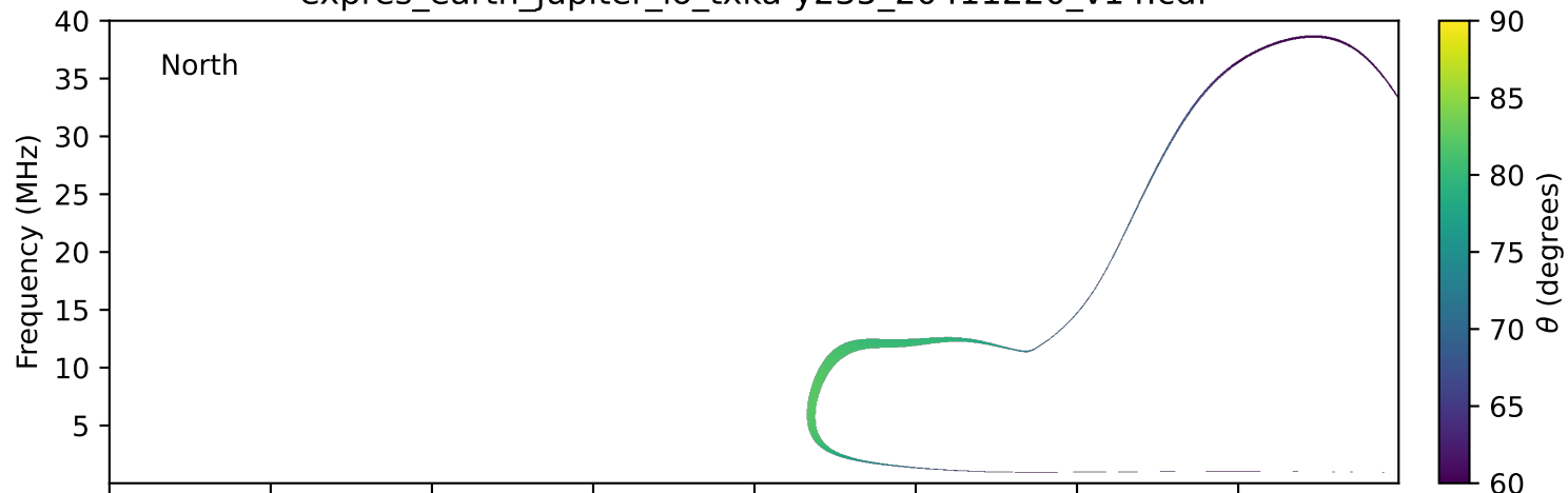
expres_earth_jupiter_io_txka-y235_20411220_v14.cdf
