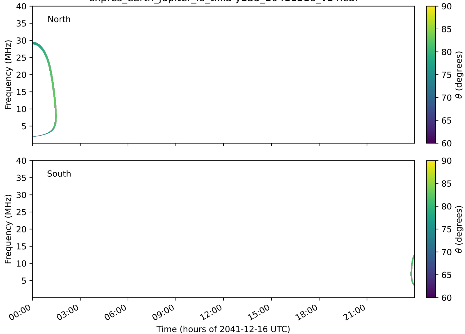
expres_earth_jupiter_io_txka-y235_20411216_v14.cdf
