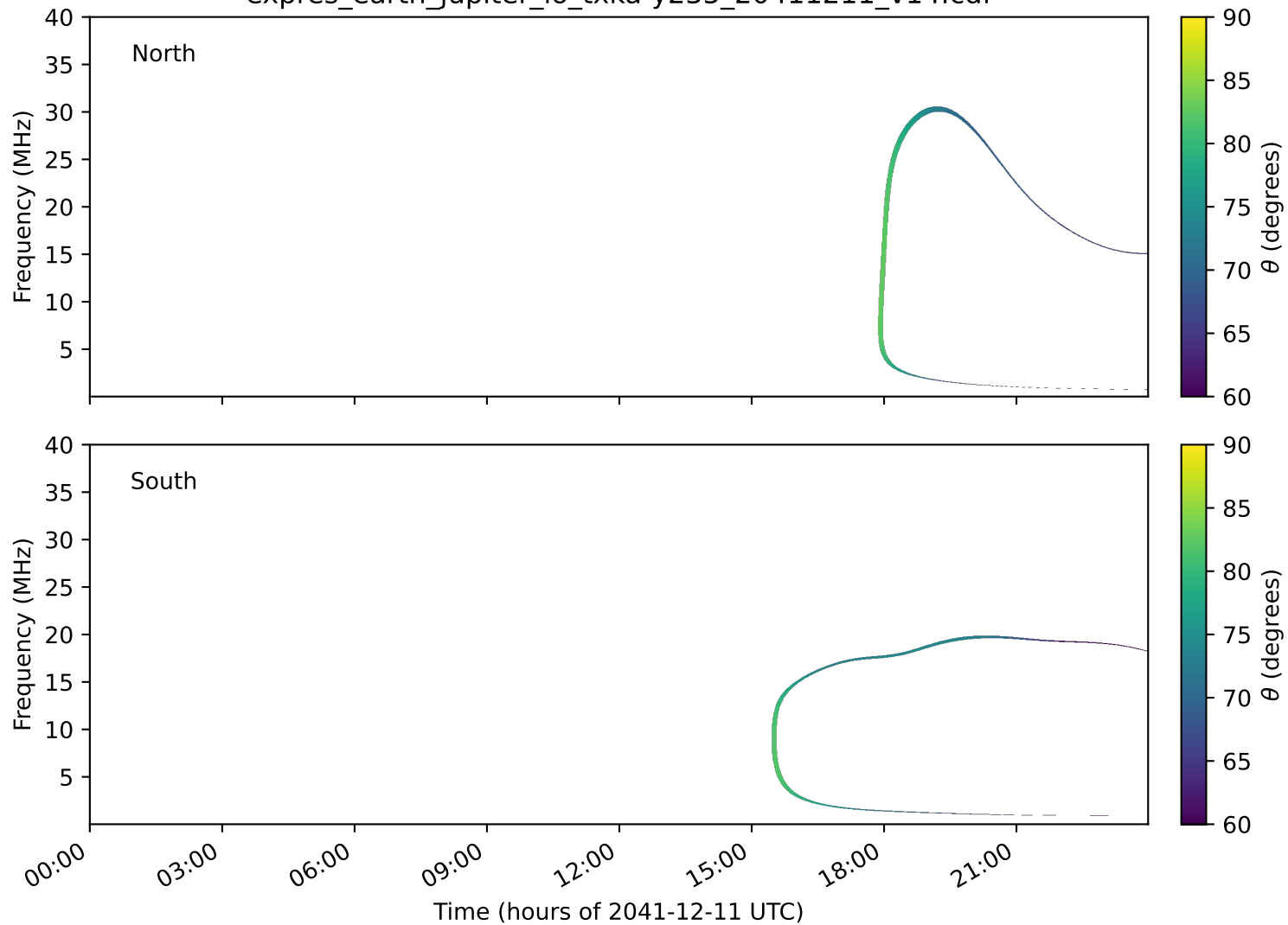
expres_earth_jupiter_io_txka-y235_20411211_v14.cdf
