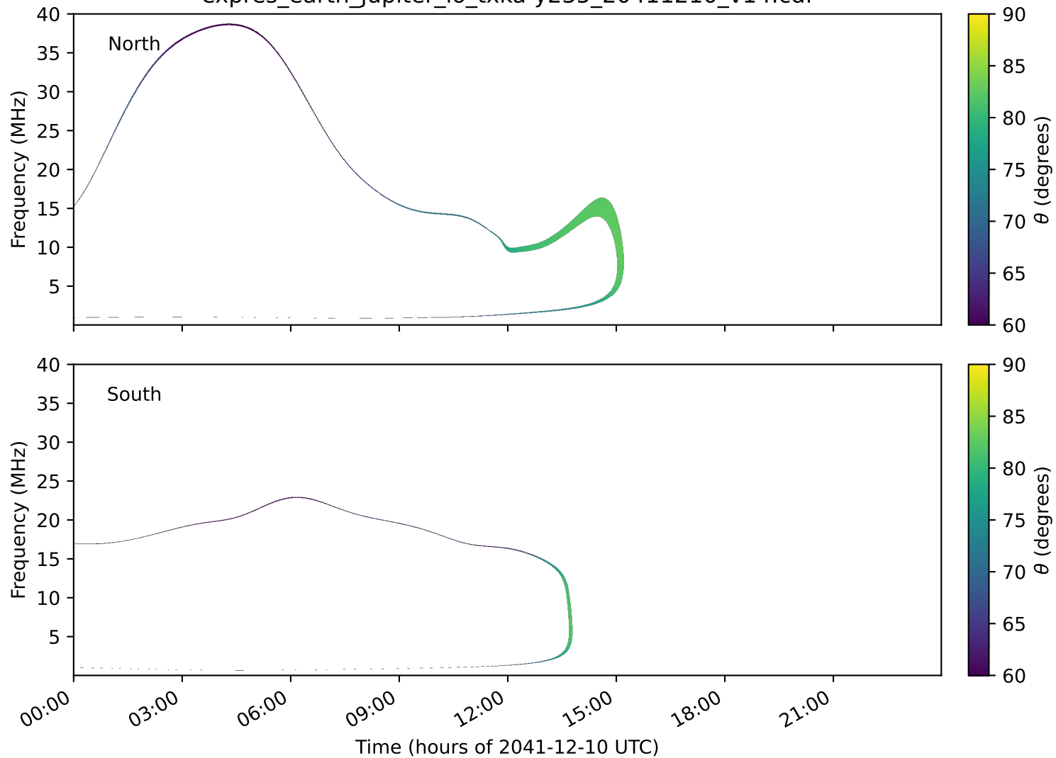
expres_earth_jupiter_io_txka-y235_20411210_v14.cdf
