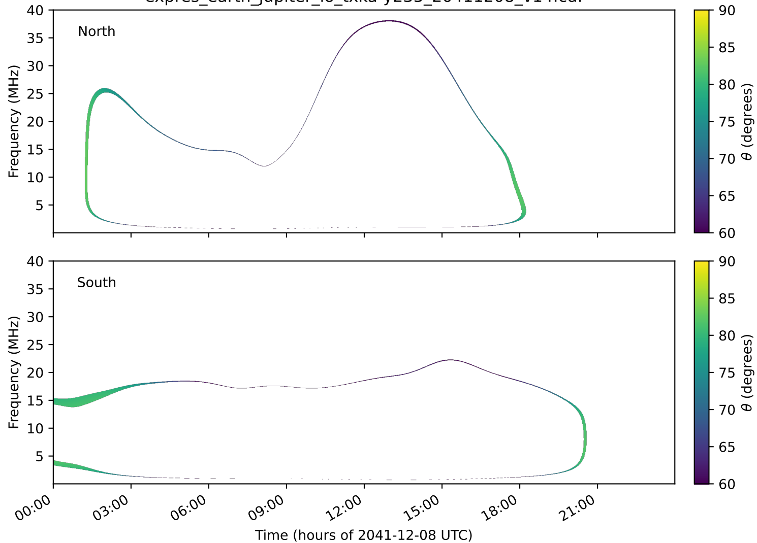
expres_earth_jupiter_io_txka-y235_20411208_v14.cdf
