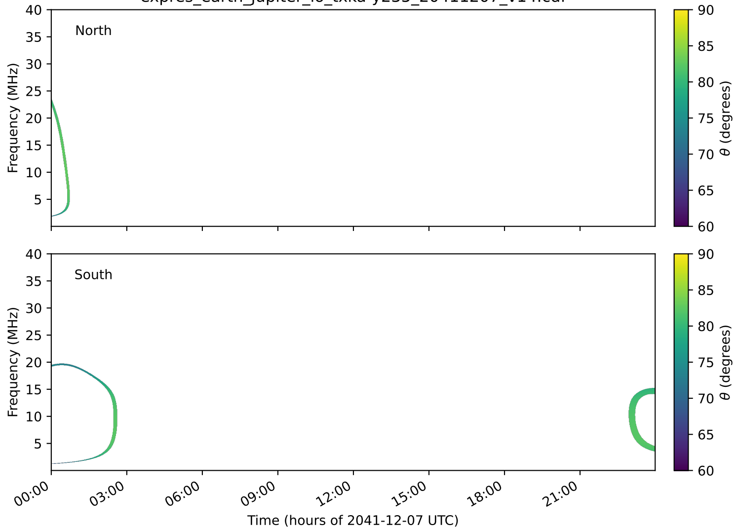
expres_earth_jupiter_io_txka-y235_20411207_v14.cdf
