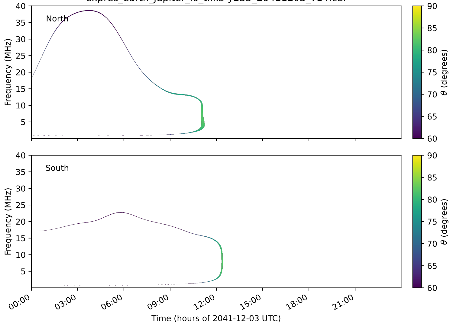
expres_earth_jupiter_io_txka-y235_20411203_v14.cdf
