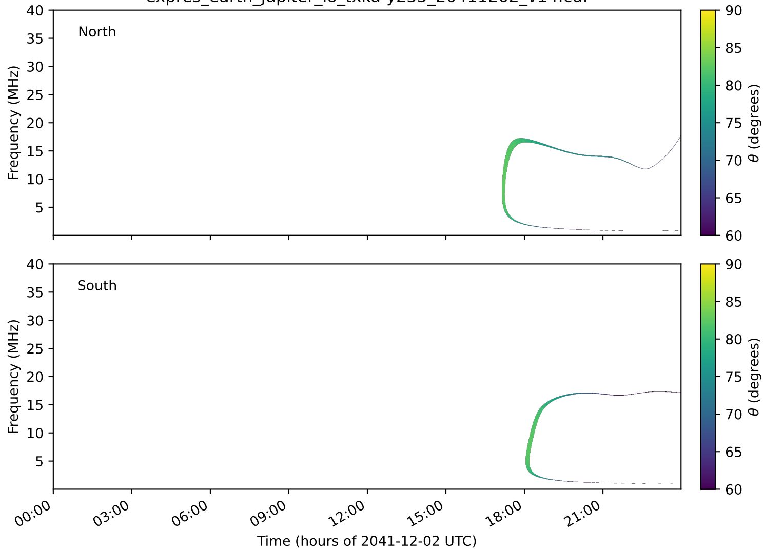
expres_earth_jupiter_io_txka-y235_20411202_v14.cdf
