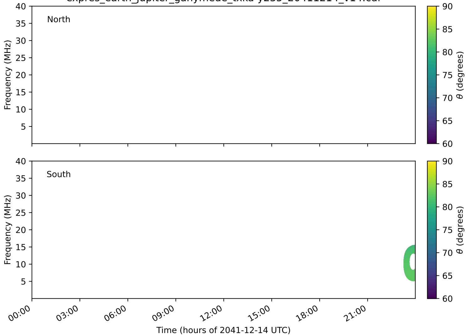
expres_earth_jupiter_ganymede_txka-y235_20411214_v14.cdf
