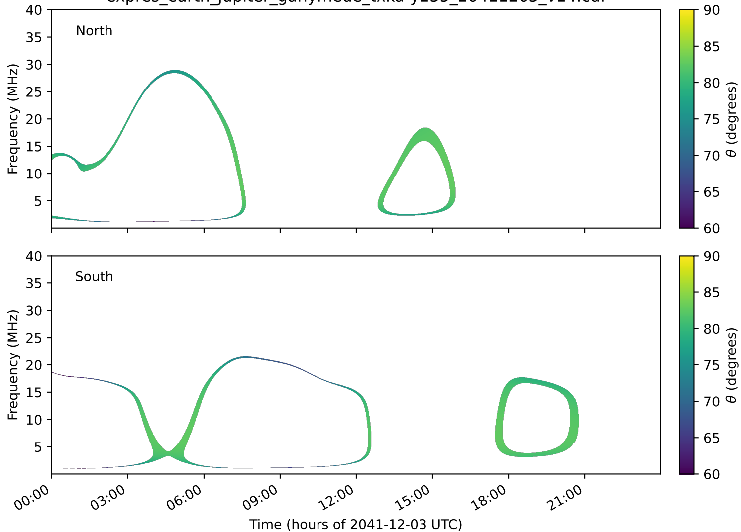
expres_earth_jupiter_ganymede_txka-y235_20411203_v14.cdf
