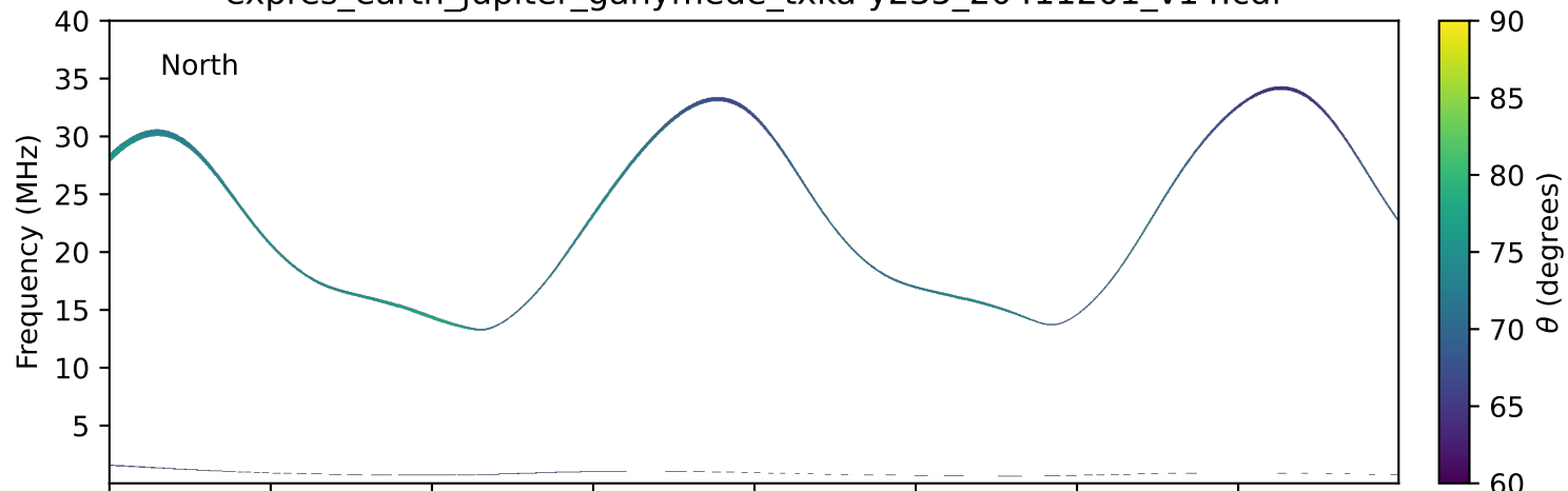
expres_earth_jupiter_ganymede_txka-y235_20411201_v14.cdf
