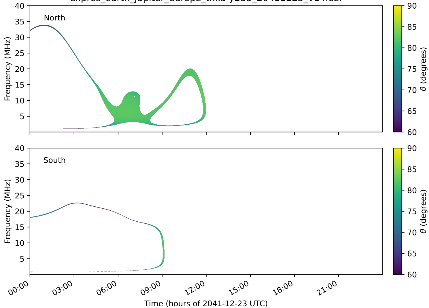
expres_earth_jupiter_europa_txka-y235_20411223_v14.cdf
