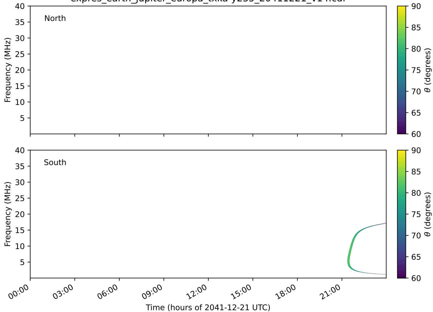
expres_earth_jupiter_europa_txka-y235_20411221_v14.cdf
