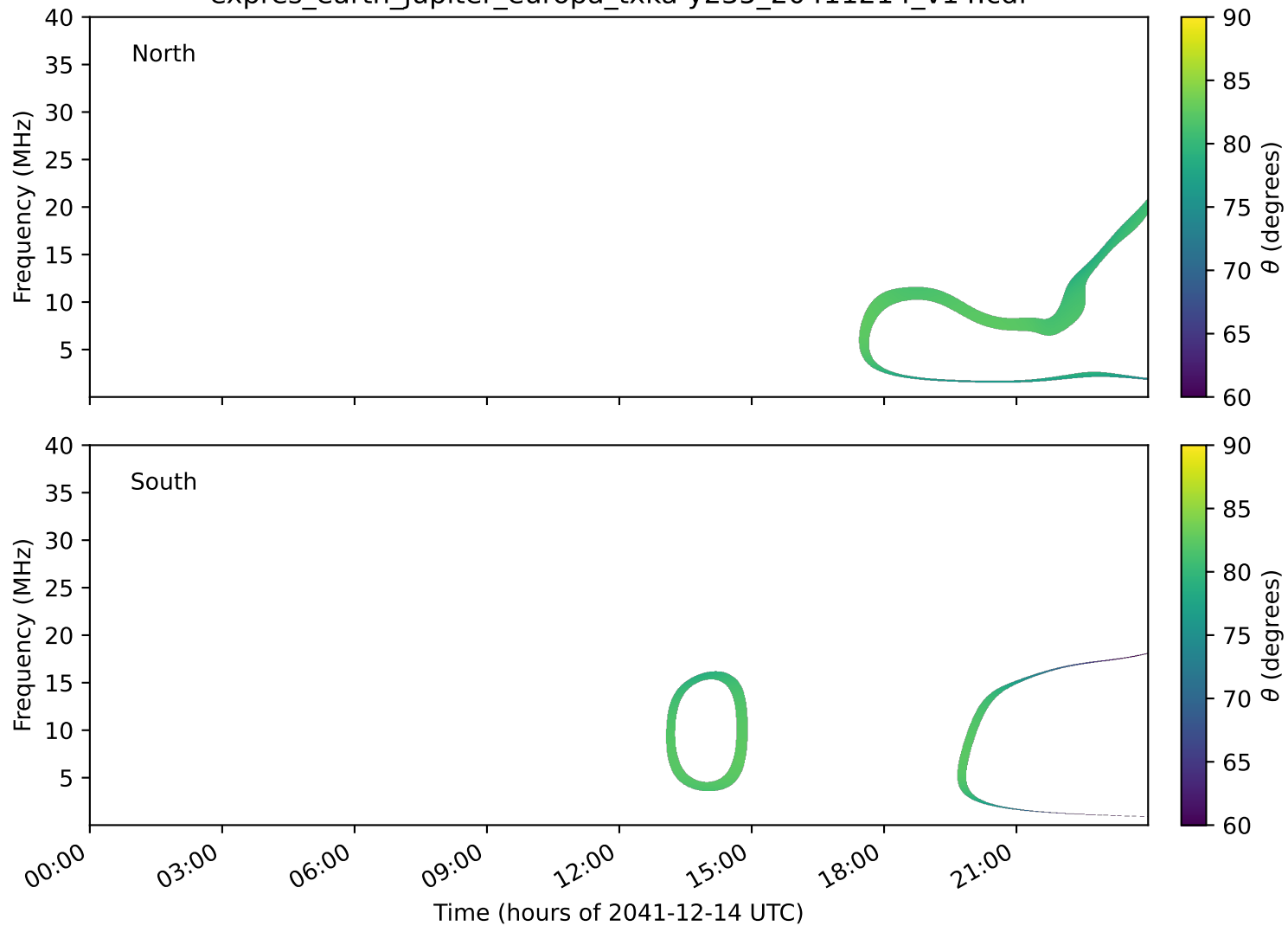
expres_earth_jupiter_europa_txka-y235_20411214_v14.cdf
