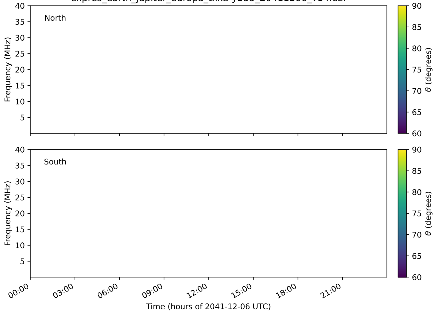
expres_earth_jupiter_europa_txka-y235_20411206_v14.cdf
