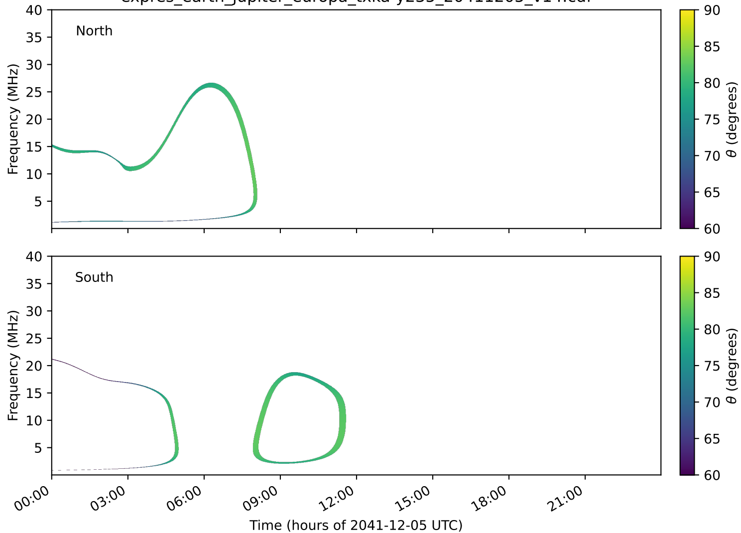
expres_earth_jupiter_europa_txka-y235_20411205_v14.cdf
