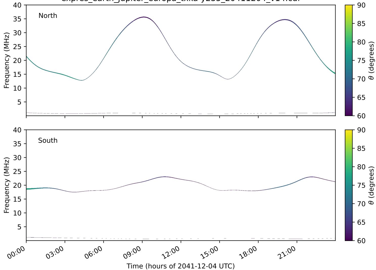
expres_earth_jupiter_europa_txka-y235_20411204_v14.cdf
