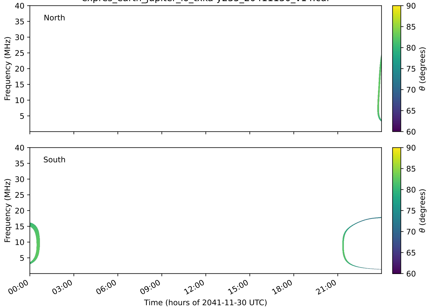
expres_earth_jupiter_io_txka-y235_20411130_v14.cdf
