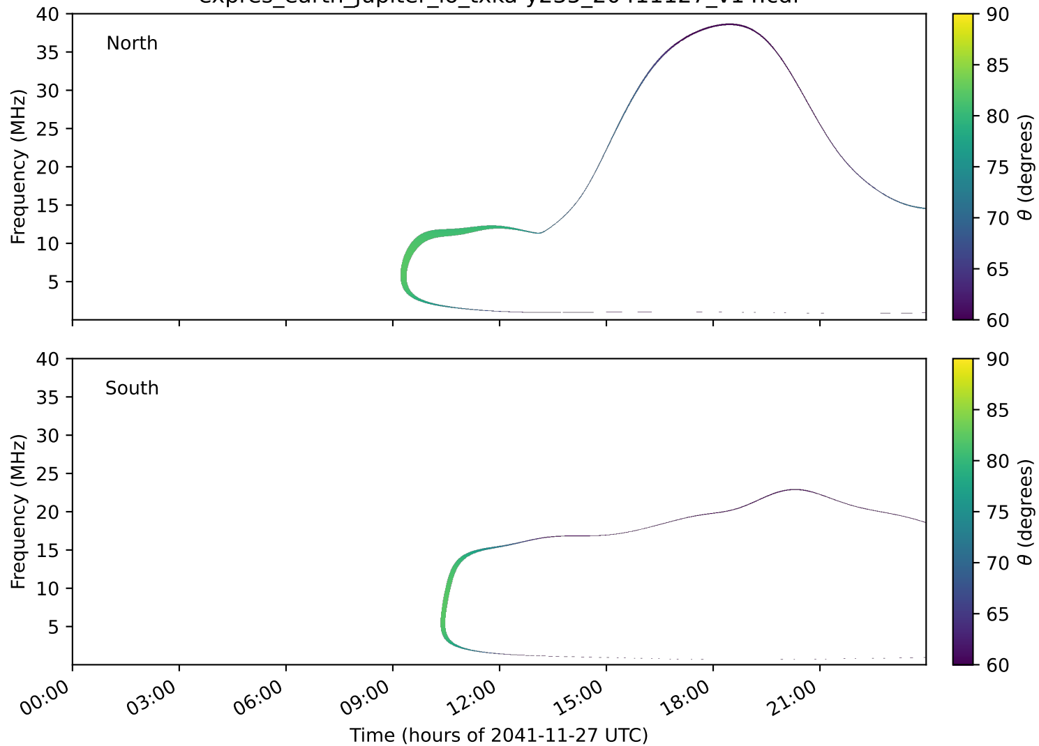
expres_earth_jupiter_io_txka-y235_20411127_v14.cdf
