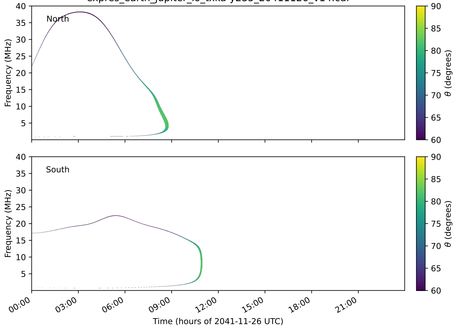
expres_earth_jupiter_io_txka-y235_20411126_v14.cdf
