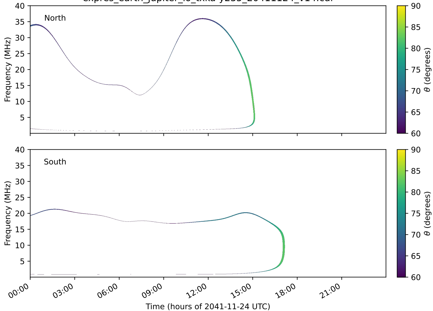
expres_earth_jupiter_io_txka-y235_20411124_v14.cdf
