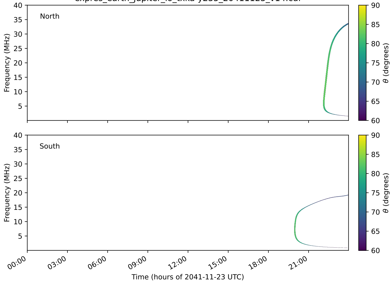
expres_earth_jupiter_io_txka-y235_20411123_v14.cdf
