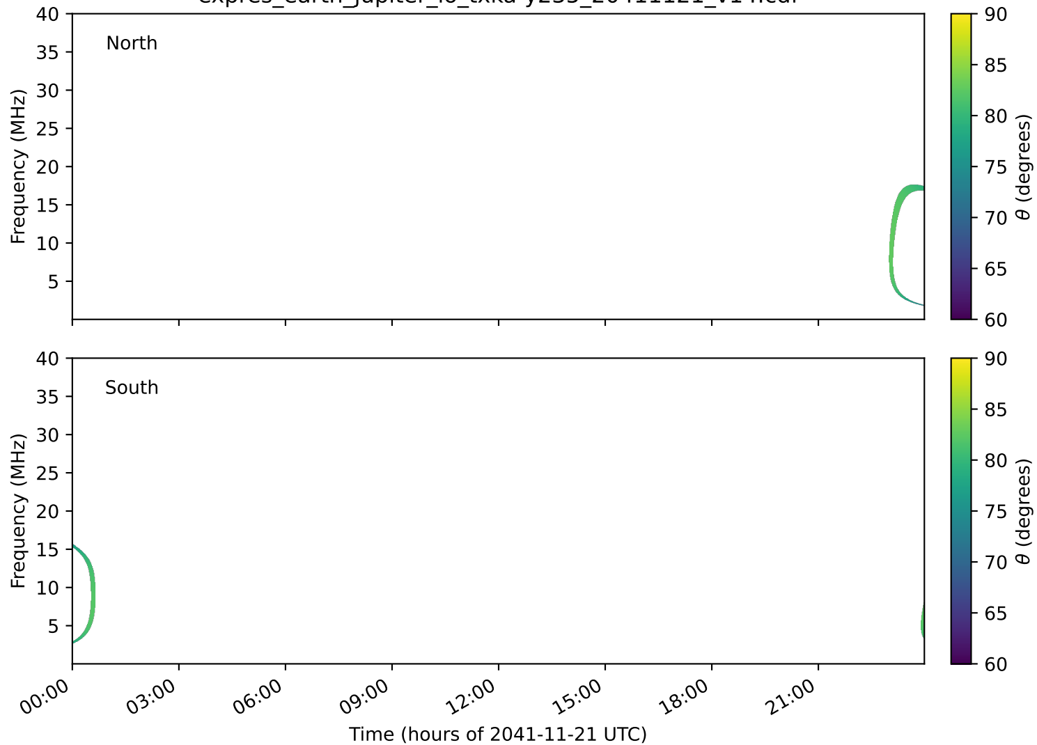
expres_earth_jupiter_io_txka-y235_20411121_v14.cdf
