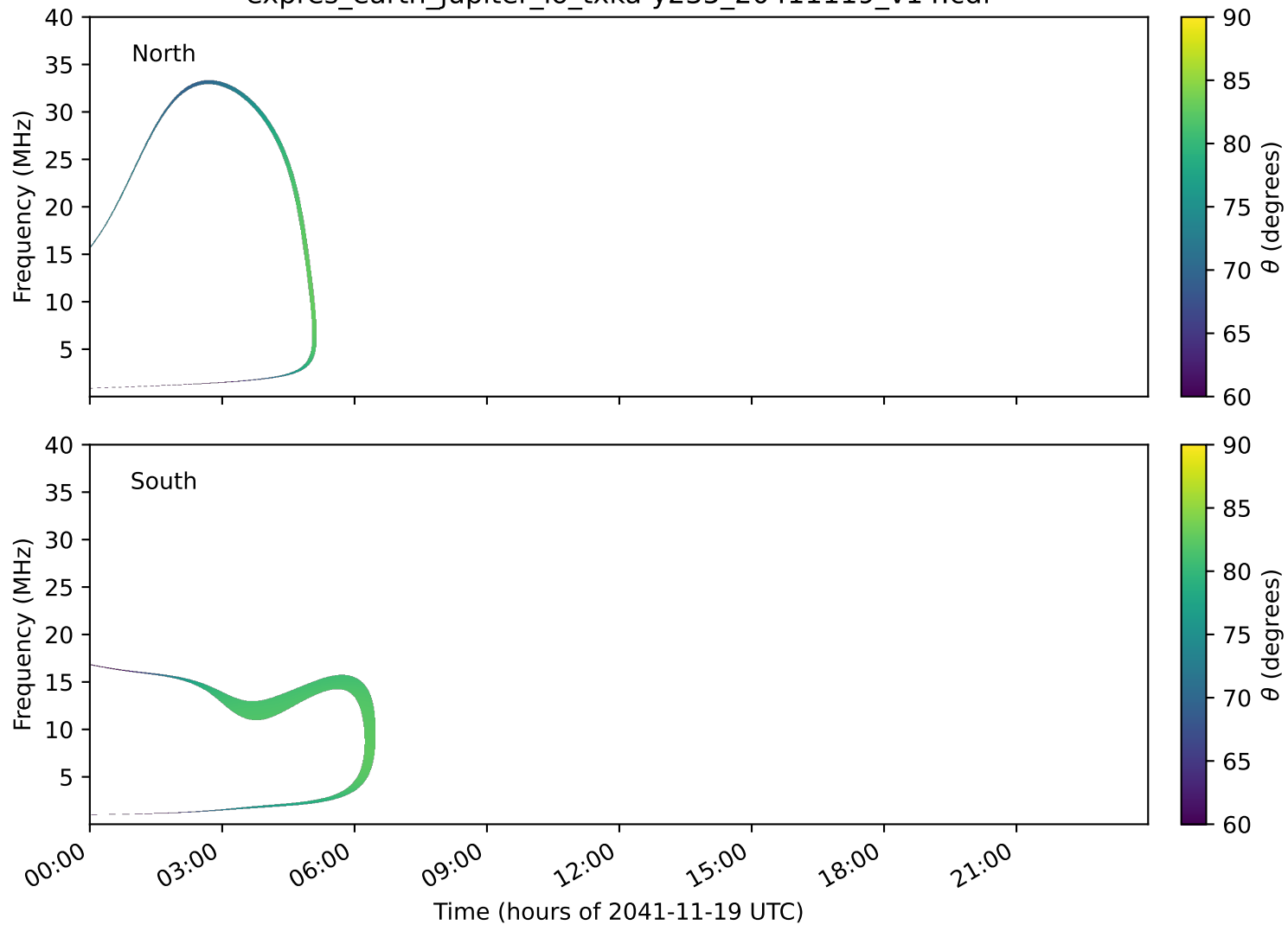
expres_earth_jupiter_io_txka-y235_20411119_v14.cdf
