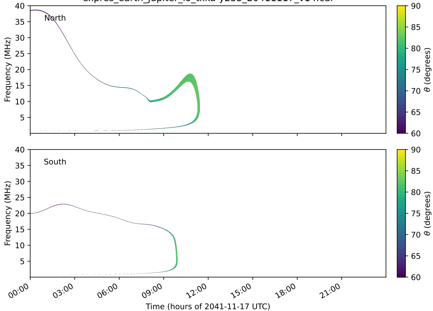
expres_earth_jupiter_io_txka-y235_20411117_v14.cdf
