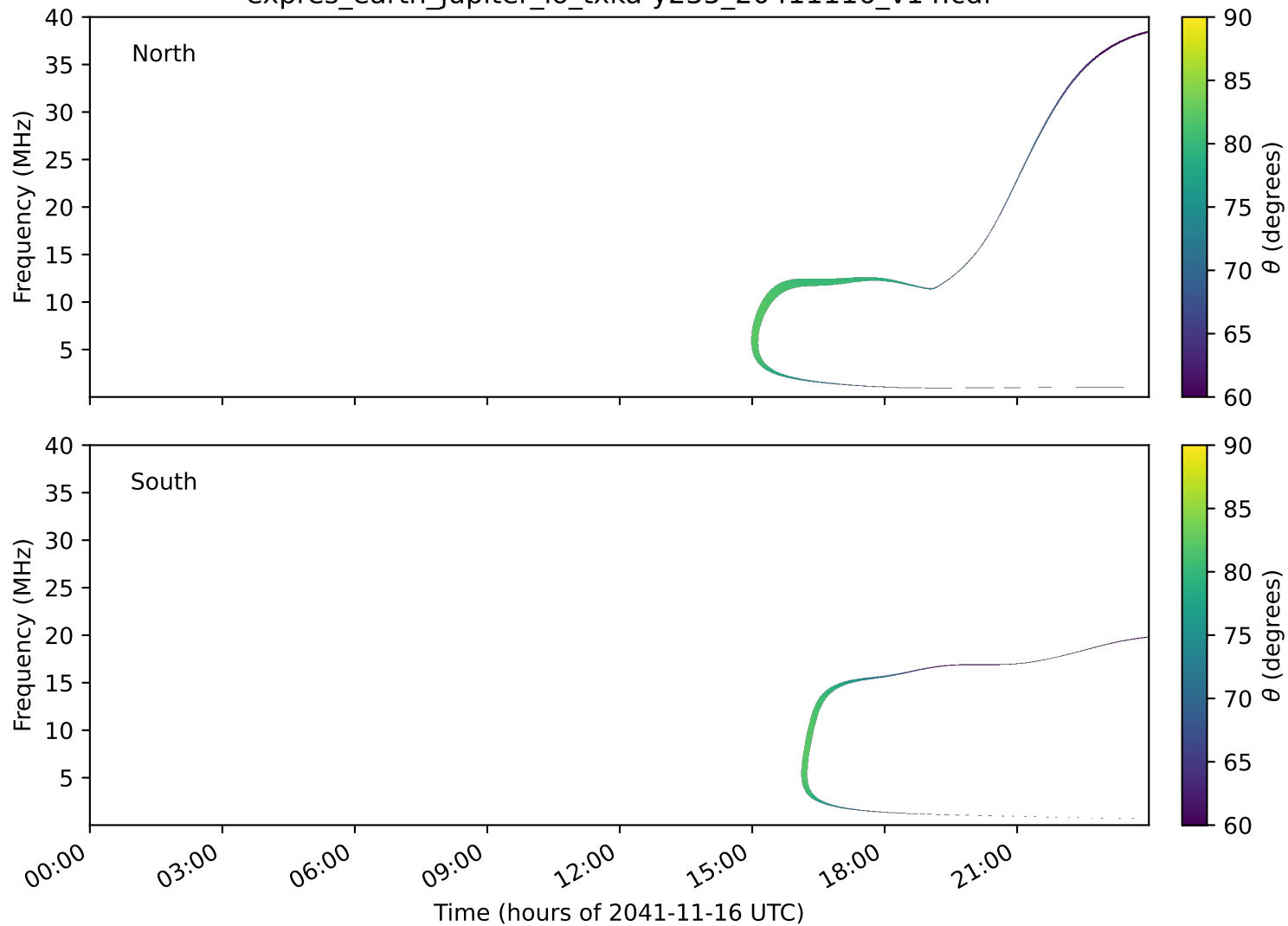
expres_earth_jupiter_io_txka-y235_20411116_v14.cdf
