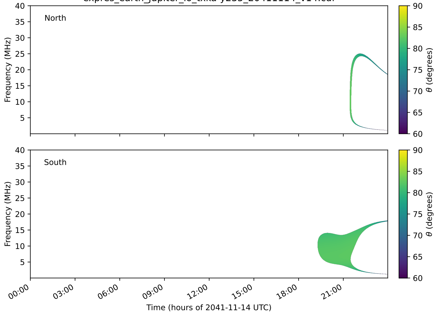
expres_earth_jupiter_io_txka-y235_20411114_v14.cdf
