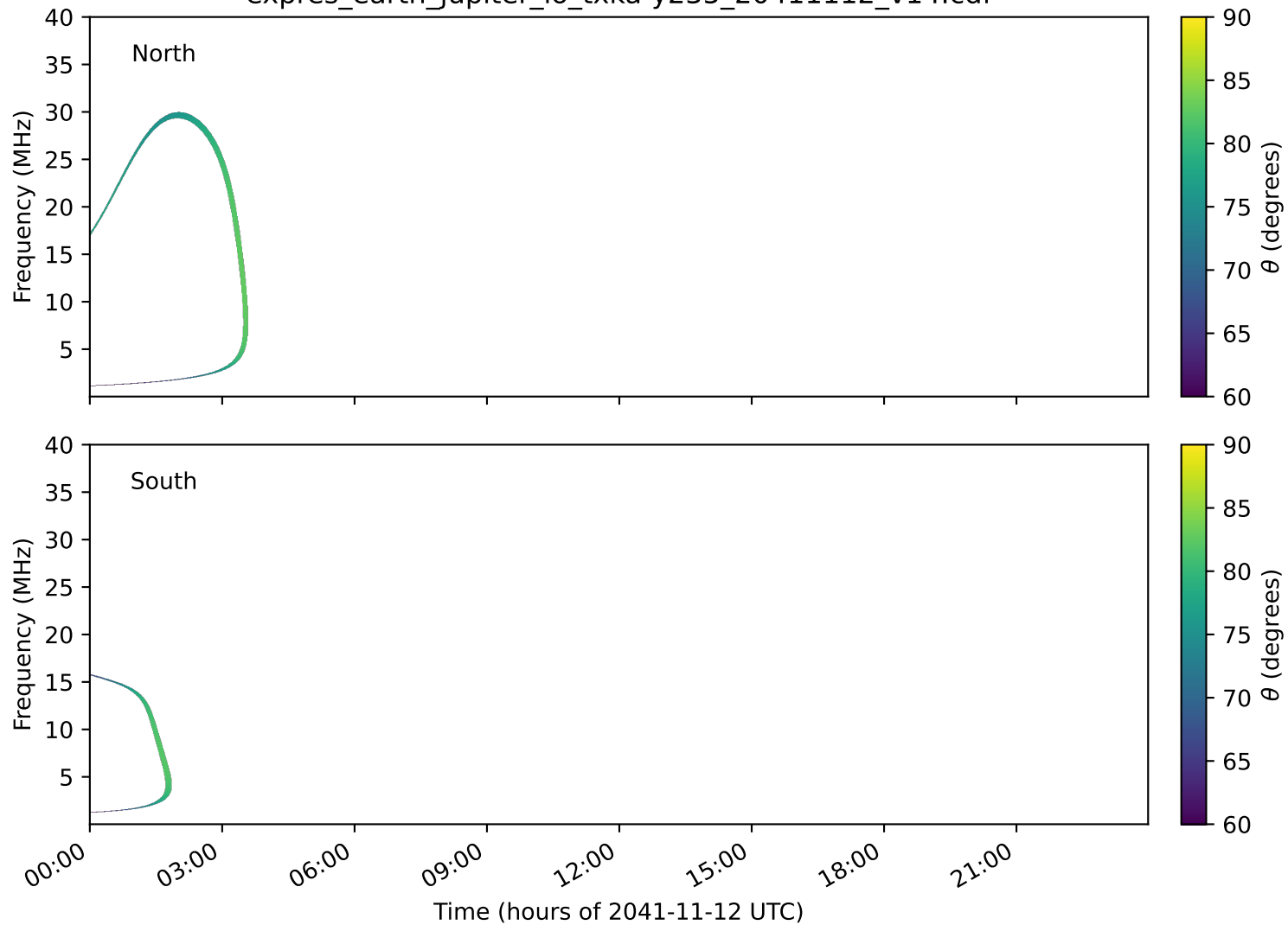
expres_earth_jupiter_io_txka-y235_20411112_v14.cdf
