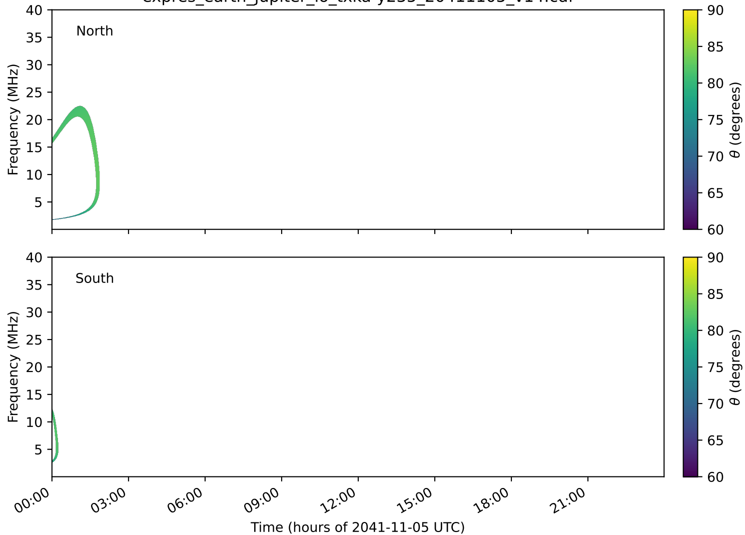
expres_earth_jupiter_io_txka-y235_20411105_v14.cdf
