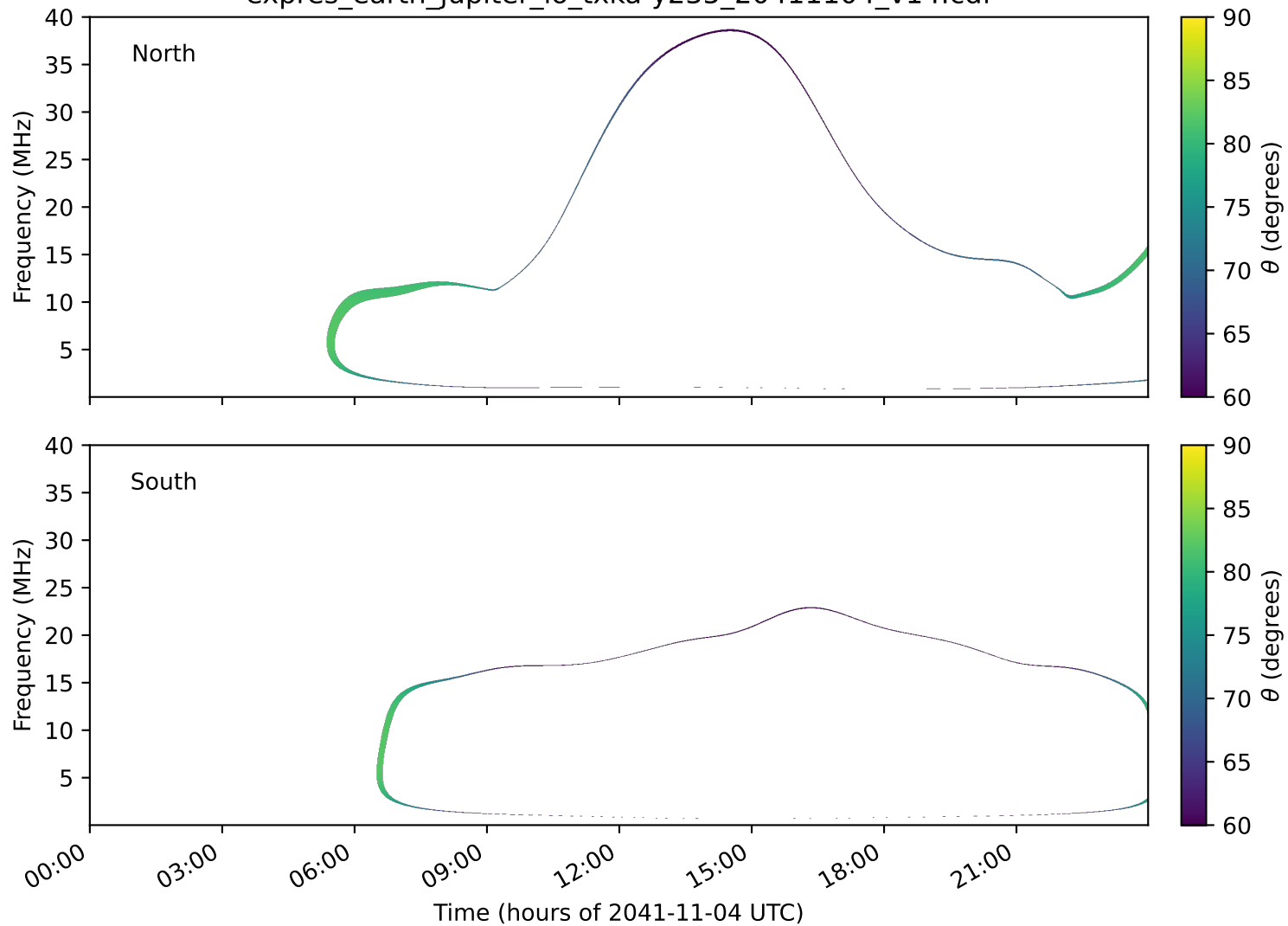
expres_earth_jupiter_io_txka-y235_20411104_v14.cdf
