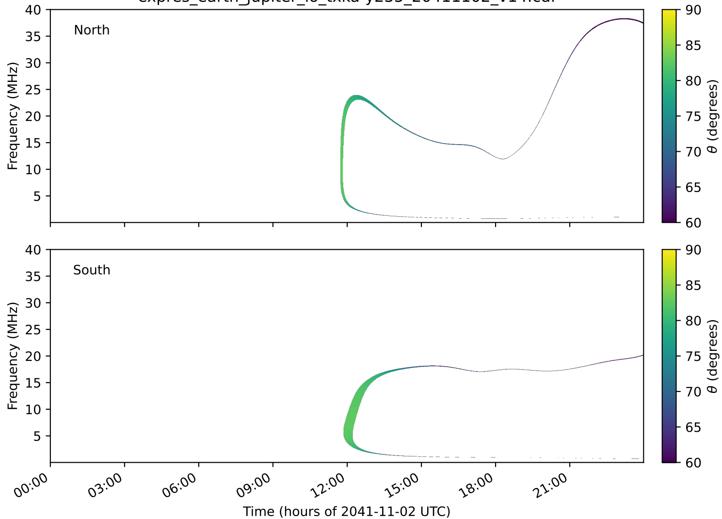
expres_earth_jupiter_io_txka-y235_20411102_v14.cdf
