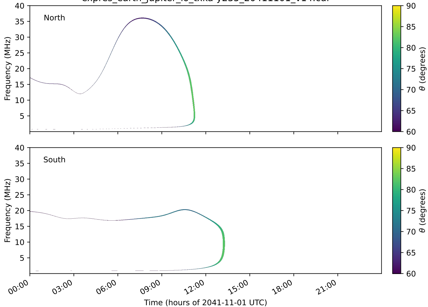
expres_earth_jupiter_io_txka-y235_20411101_v14.cdf
